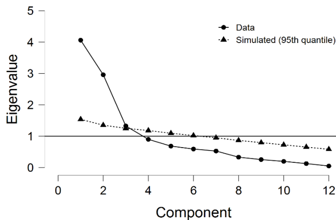
Figure 1. Scree plot
