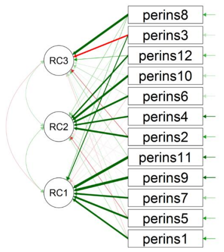
Figure 2. Path diagram of governance of violence
