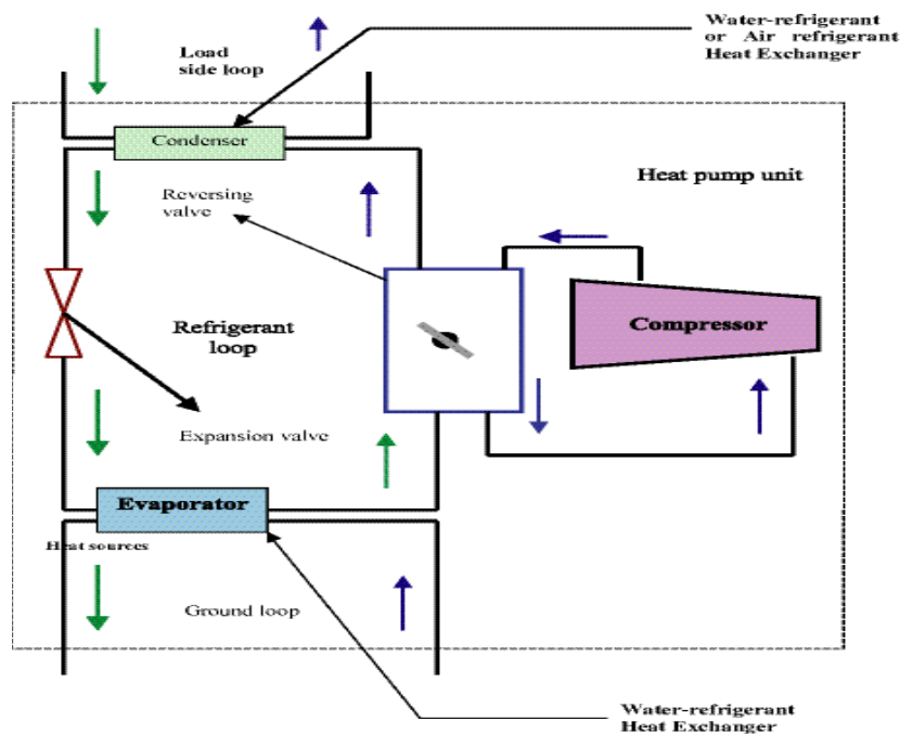
Figure 8. Schematic of GSHP system (heating mode operation).
