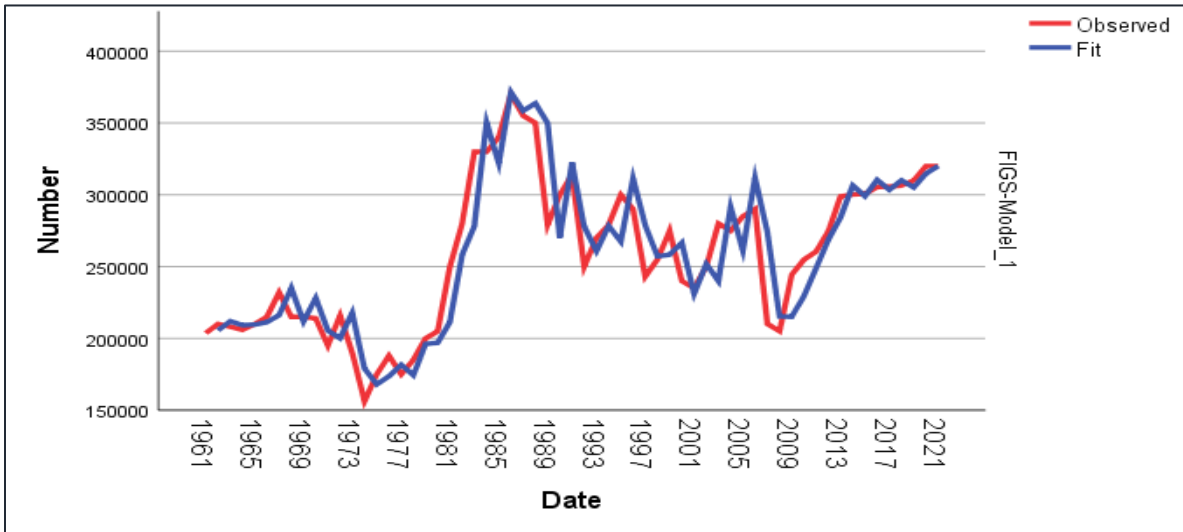
Figure 3. 5. Predicted value and actual values of cherry production time series by using ARIMA (0,1,3)
