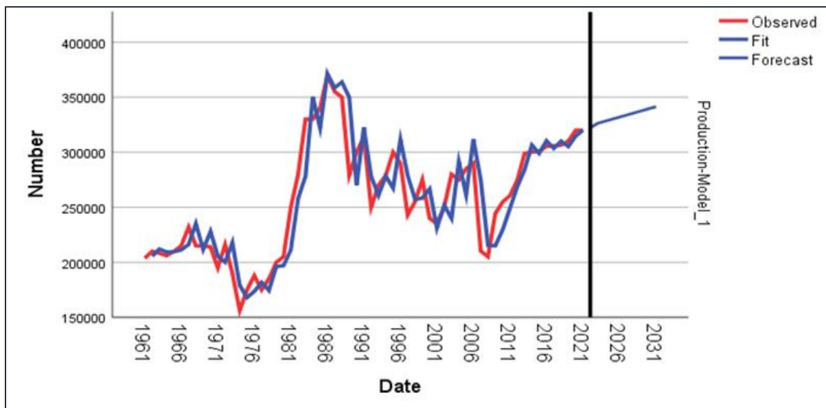
Figure 3.6. Predicted values of figs production in 2021
