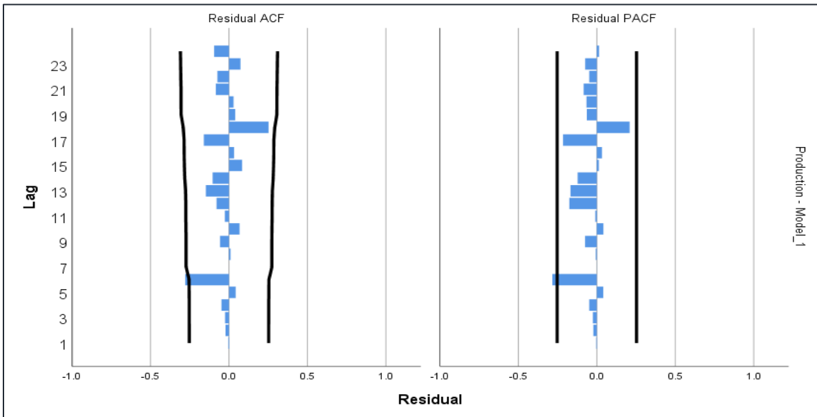
Figure 3. 6. Residual for ACF AND PACF (0, 1, 3)
