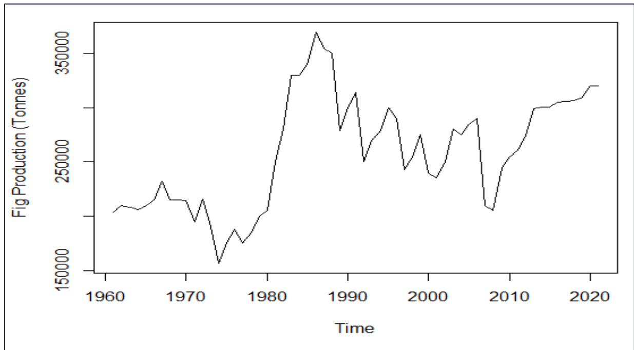
Figure 3. 1. Figs production in Turkey from 1961 to 2021
